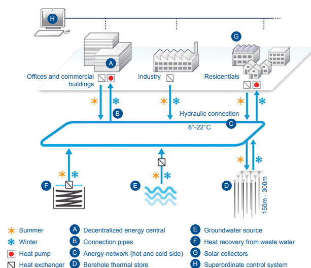
Layout of an anergy network (special form of a cold heat network) as proposed by Amstein & Walther.
